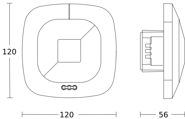
Dimension Drawing 1
